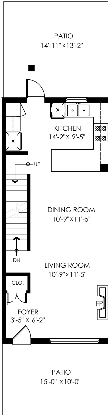
Main Floor Plan
