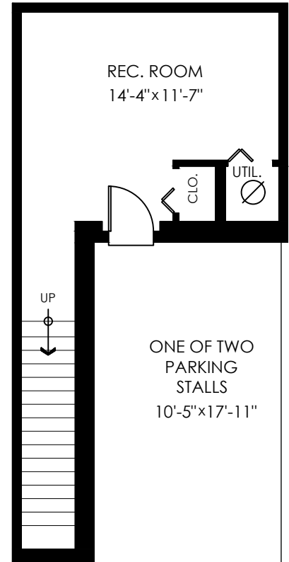
Lower Floor Plan
